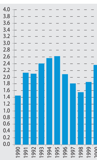
Figure 3-43: Propylene use
