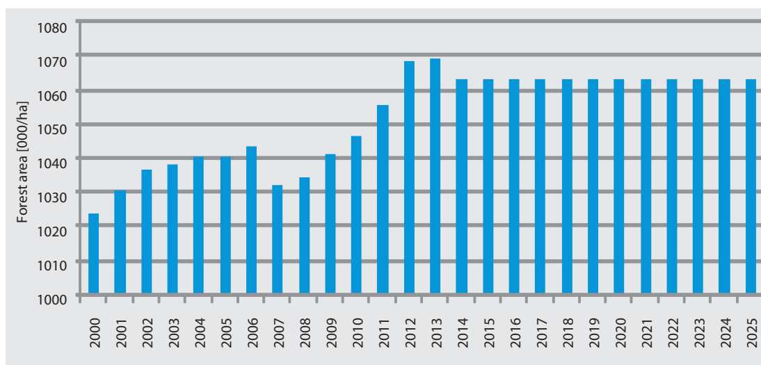
Figure 5-50: Forest area
