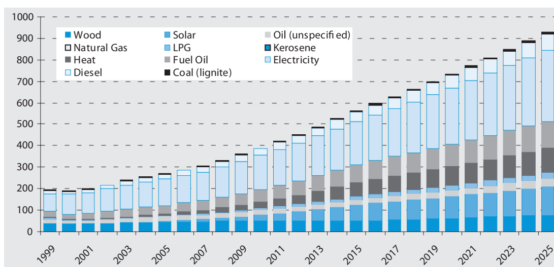
Figure 5-8: Trend of energy consumption for services sector (ktOE)
