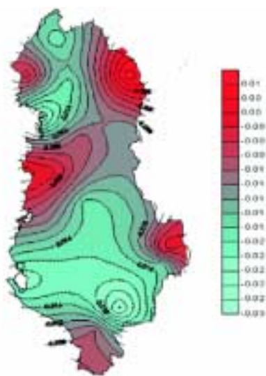
Fig.I.2 Annual temperatures (1960-1990)
